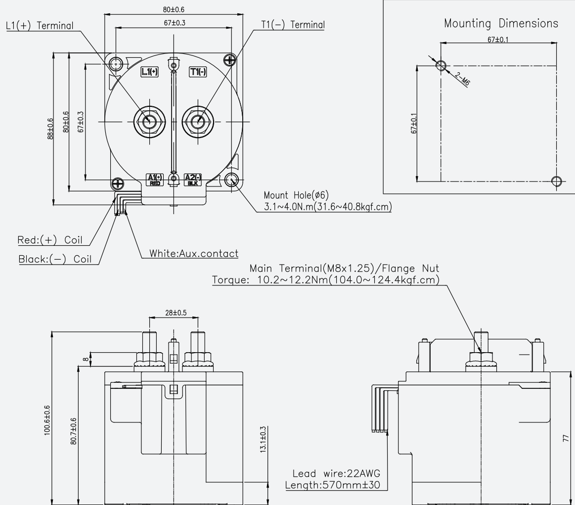
Schematic (Top View)
