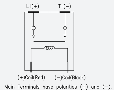
Schematic (Top View)
